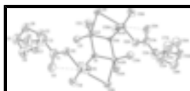
Fig. 1. The molecular structure of the title compound, showing 50% probability displacement ellipsoids. H atoms have been omitted for clarity. Symmetry code: (A) 1-x, 1-y, 2-z.
